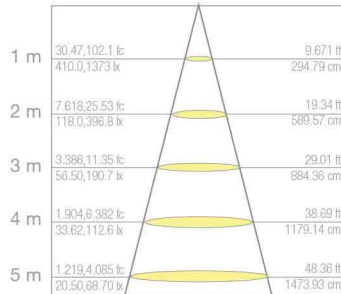
Konik Diyagram ( 35 W 4000K )
